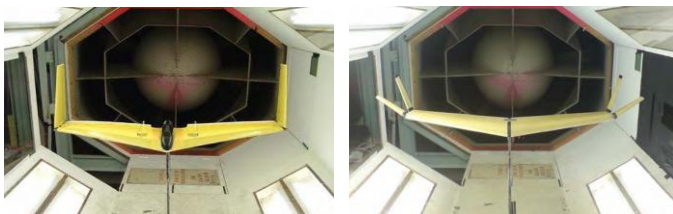
Fig. 4. Active winglet concept for drag reduction [4].
