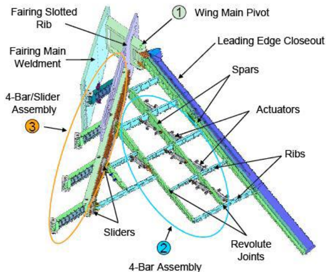
Fig. 9. Mechanism employed by NextGen in its "variable sweep, variable chord" concept [1].
