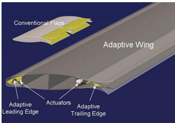
Fig. 5. FlexSys' "compliant wing concept" [9].
