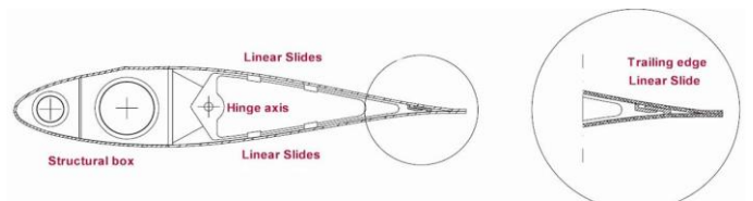
Fig. 6. DLR finger concept [12].
